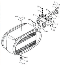
C-130 OIL COOLER PN L8602772-1
